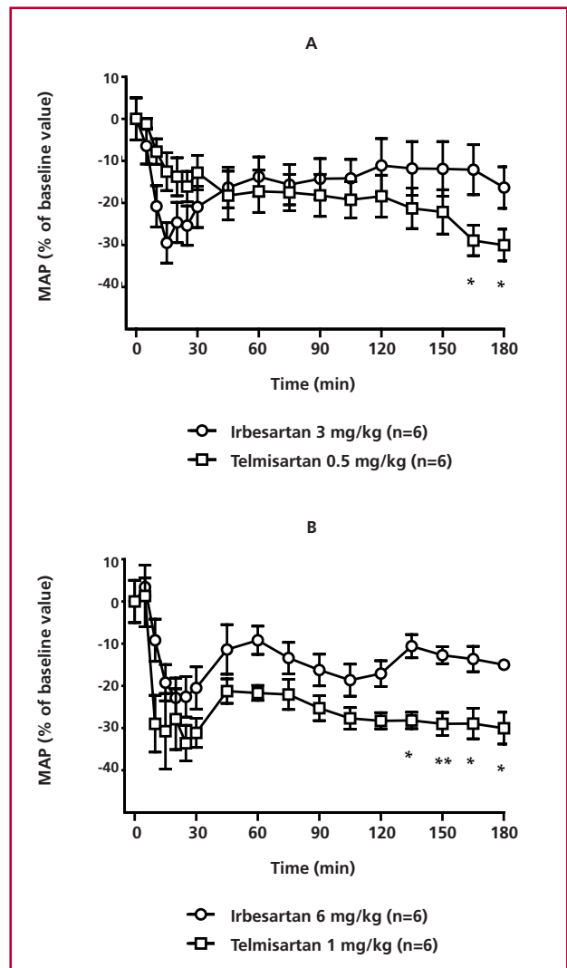
Fig. 1. Time course of mean arterial pressure change ( \Delta MAP, % of baseline values), after telmisartan 0.5 or 1 mg/kg or irbesartan 3 or 6 mg/kg in spontaneously hypertensive rats. Each point shows mean ± SEM of six rats. * p < 0.05 vs. irbesartan (two-way ANOVA followed by the Bonferroni test).
